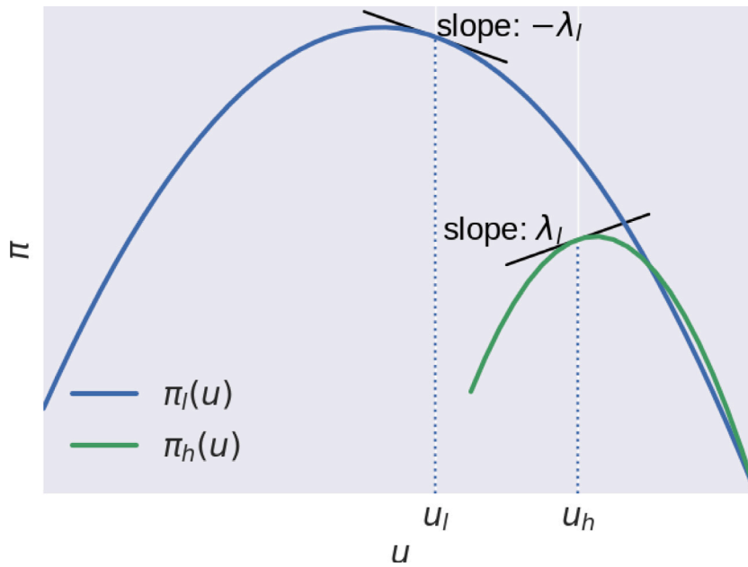
Fig. 1. Insurer's profits \pi_l(u), \pi_h(u) as a function of u .
